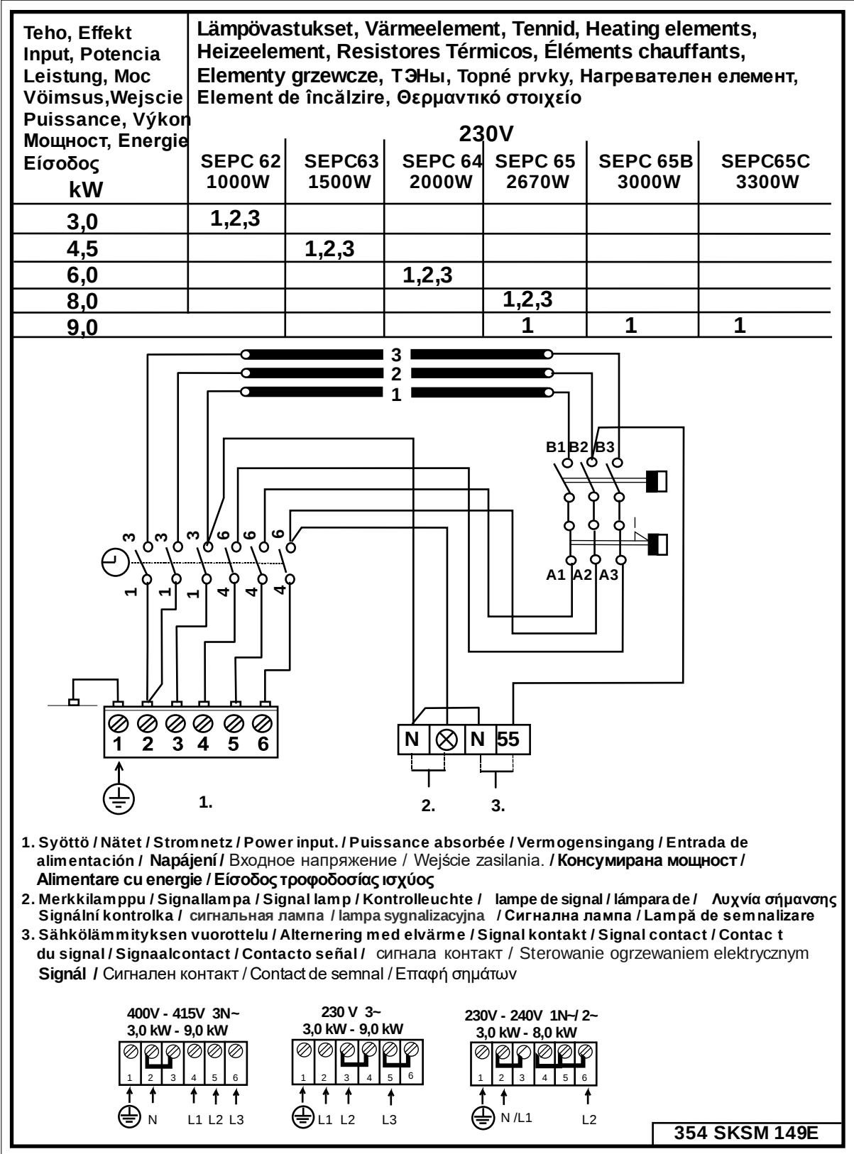
Image 4 Viring diagram
